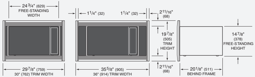
Model MWC24 with L Series trim
