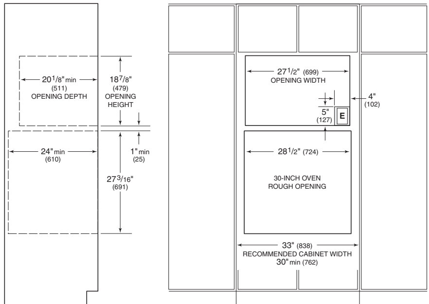
Installation with 36" L Series trim
