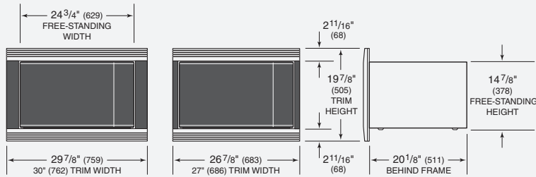
Model MWC24 with E Series trim
