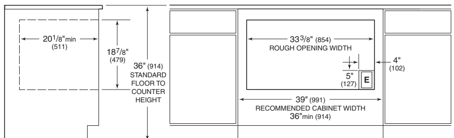
Installation with 36" L Series trim
