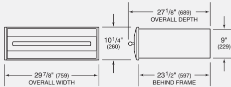
Model WWD30 with L Series drawer front
