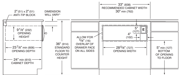
ANTI-TIP BLOCK APPLICATION
