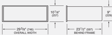
Model WWD30 with integrated drawer front
