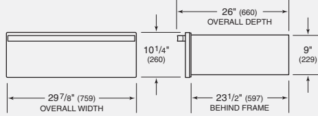
Model WWD30 with E Series drawer front
